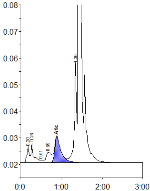
Peak table - ID: 10430790
